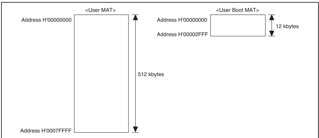
Figure 21.3 Flash Memory Configuration
