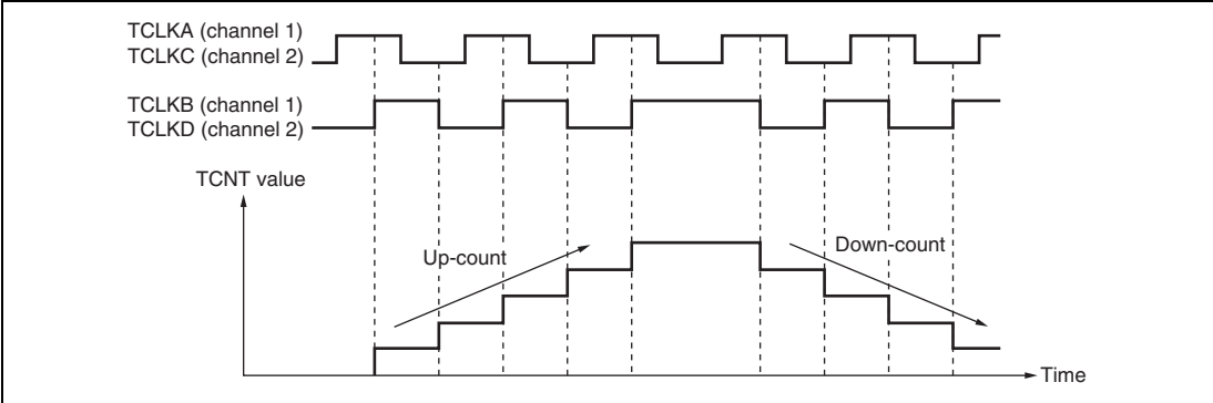
Figure 10.33 Example of Phase Counting Mode 4 Operation
