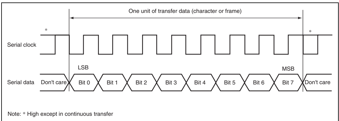
Figure 15.9 Data Format in Clocked Synchronous Communication
