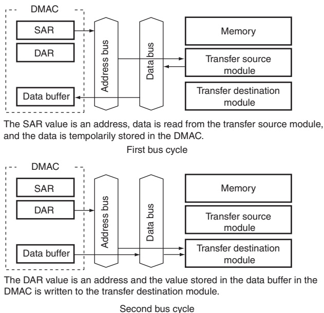
Figure 9.5 Data Flow of Dual Address Mode
