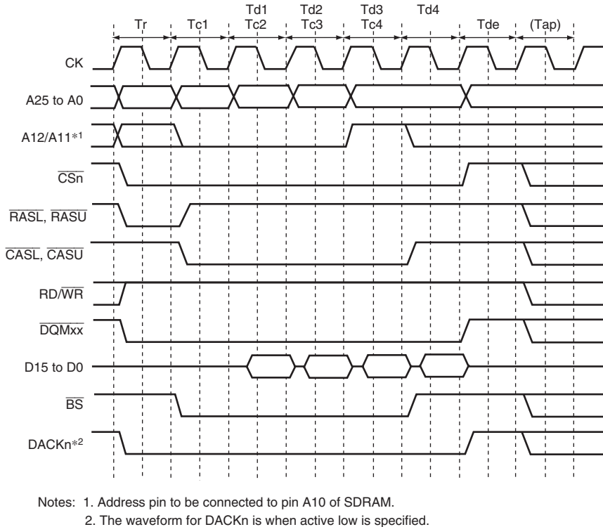
Figure 8.14 Burst Read Basic Timing (CAS Latency 1, Auto-Precharge)
