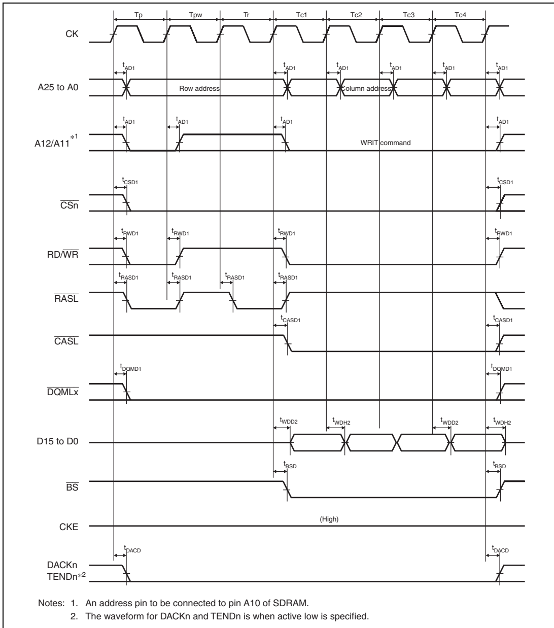
Figure 27.33 Synchronous DRAM Burst Write Bus Cycle (Four Write Cycles) (Bank Active Mode: PRE + ACT + WRITE Commands, Different Row Addresses, WTRCD = 0 Cycle, TRWL = 0 Cycle)
