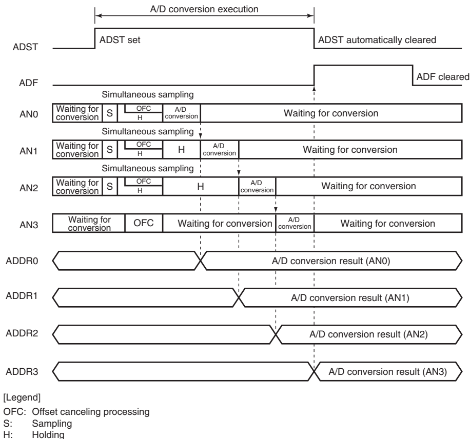
Figure 17.2 Example of A/D_0 Converter Operation (Single-Cycle Scan Mode)
