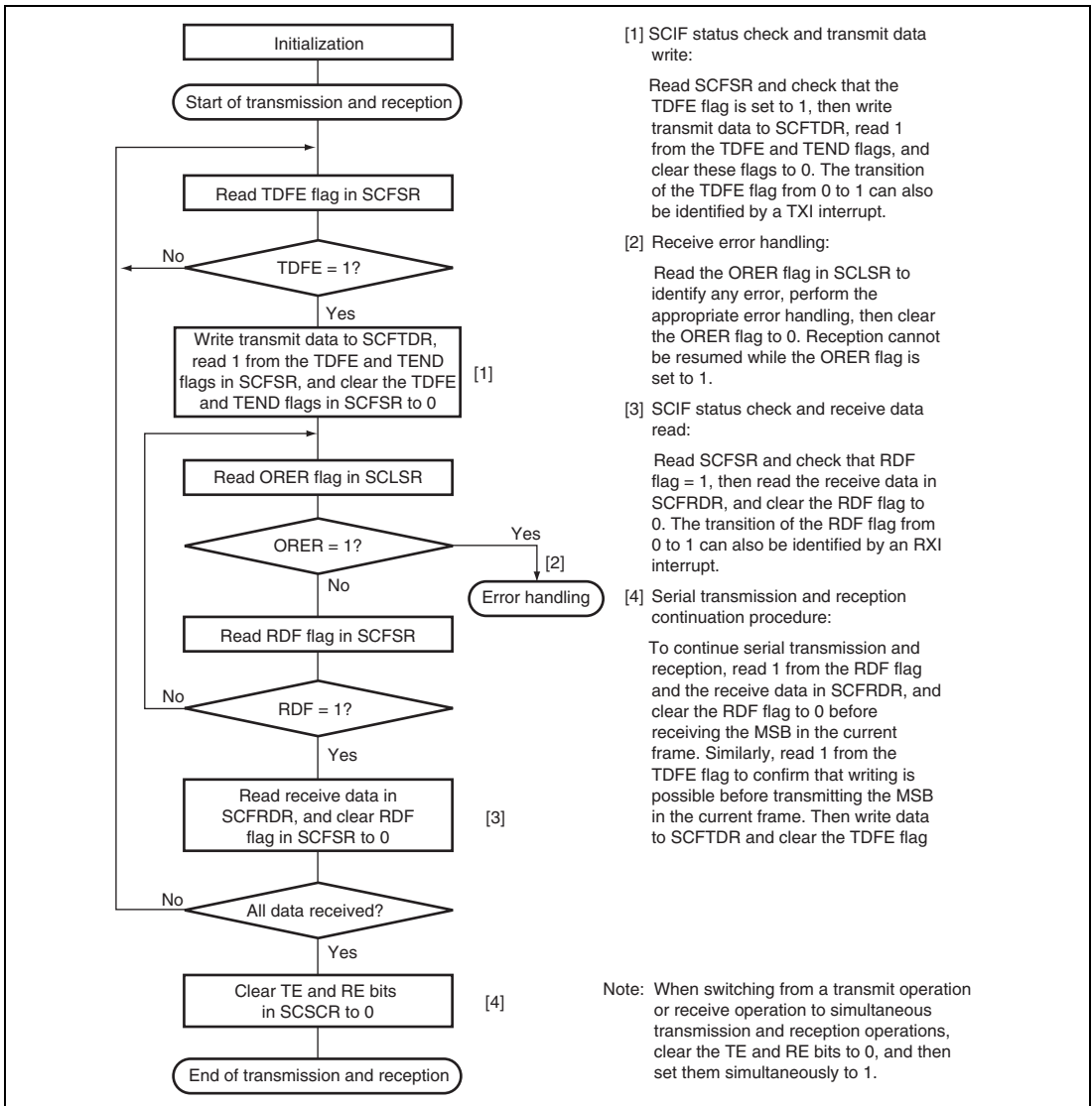
Figure 15.16 Sample Flowchart for Transmitting/Receiving Serial Data
