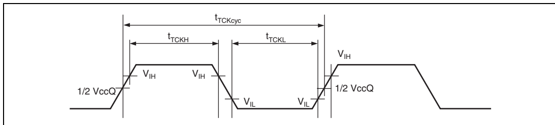
Figure 27.51 TCK Input Timing
