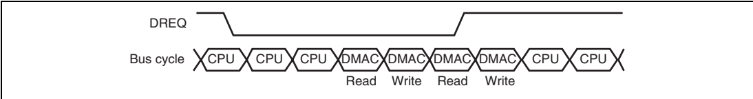
Figure 9.11 DMA Transfer Example in Burst Mode (Dual Address, DREQ Low Level Detection)
