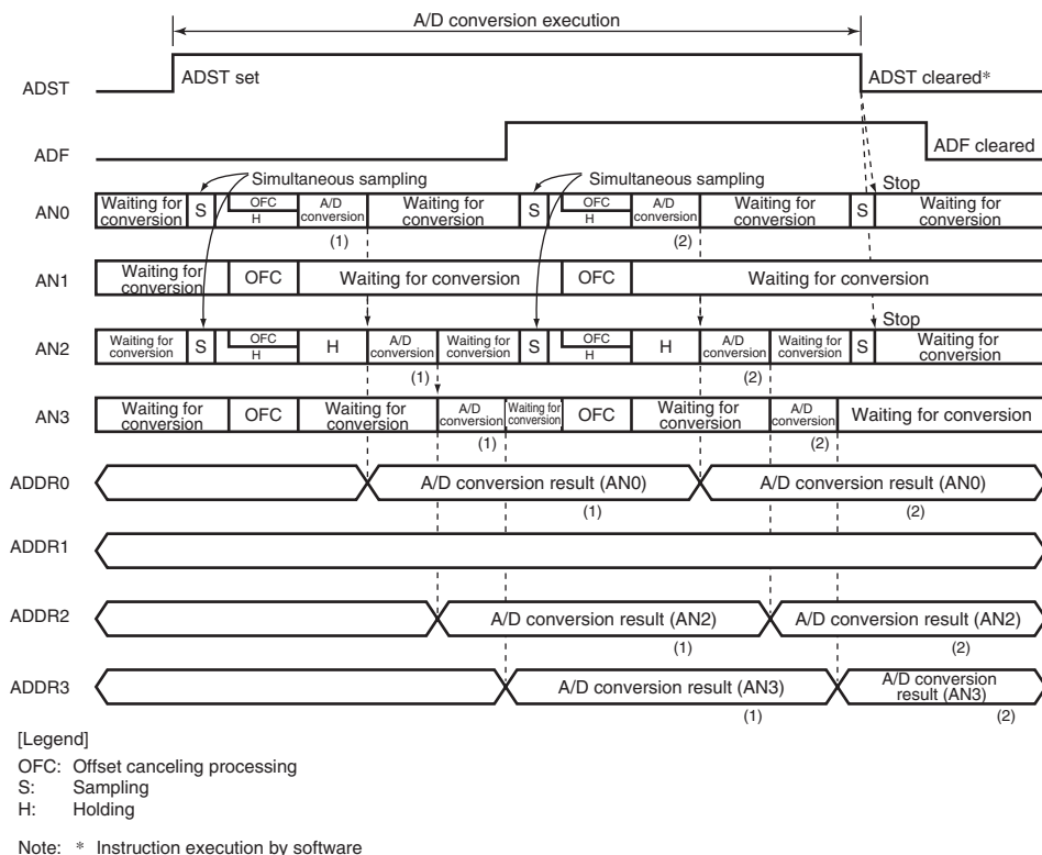
Figure 17.3 Example of A/D Converter Operation (Continuous Scan Mode)
