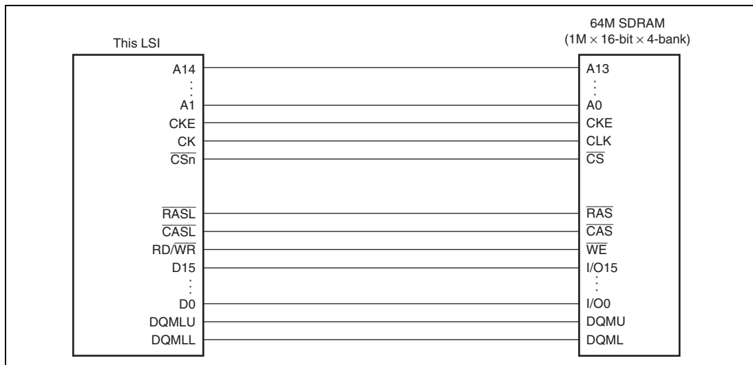
Figure 8.13 Example of 16-Bit Data Width SDRAM Connection ( RASU and CASU are Not Used)
