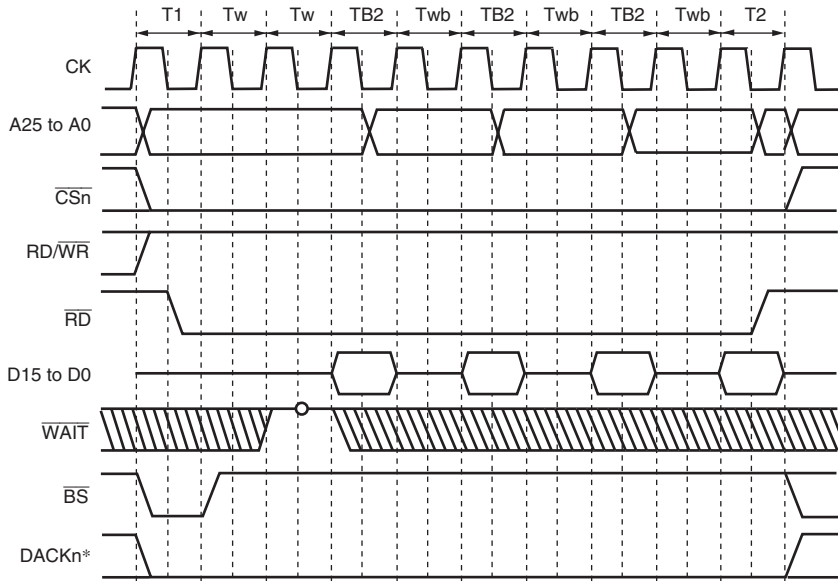
Figure 8.32 Burst ROM Access Timing (Clock Asynchronous) (Bus Width = 32 Bits, 16-Byte Transfer (Number of Burst 4), Wait Cycles Inserted in First Access = 2, Wait Cycles Inserted in Second and Subsequent Access Cycles = 1)
